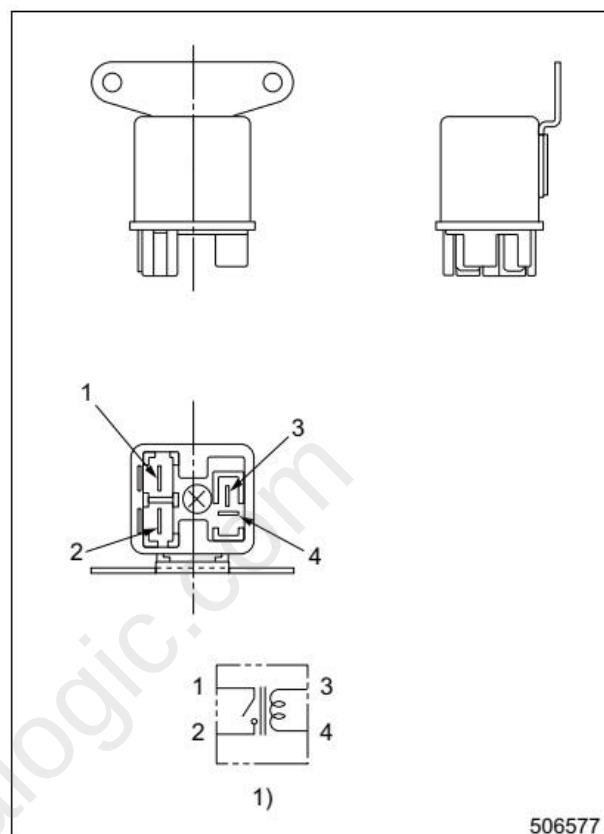
1) Connecting diagram
