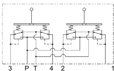
Hydraulik-symbol
