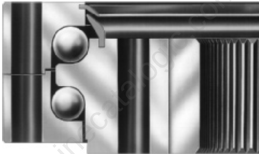
Figure 7.4 – Double Row Ball Bearing
