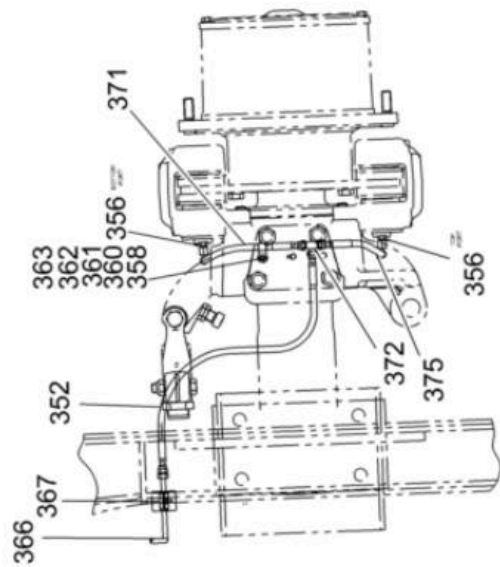
DETAIL "Q"
