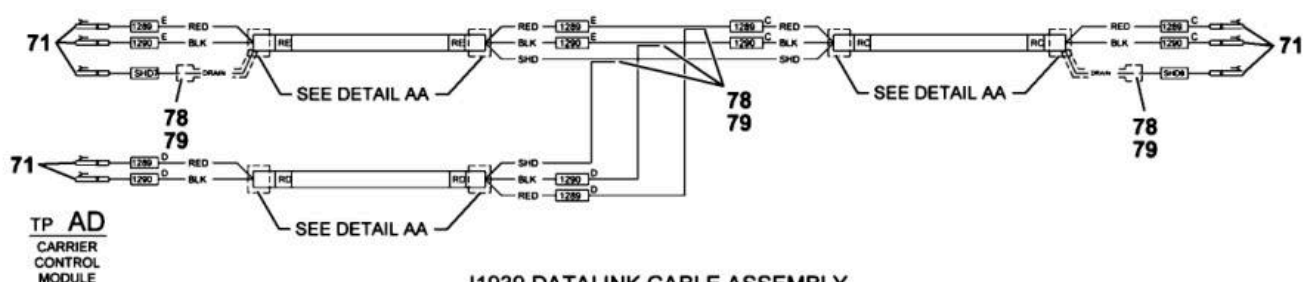
J1939 DATALINK CABLE ASSEMBLY
