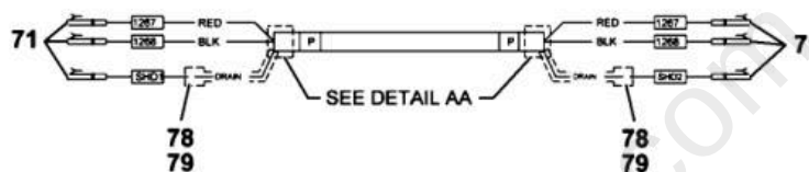
CABLE DETAIL P CONTROL MODULE PROPRIETARY DATALINK CABLE
