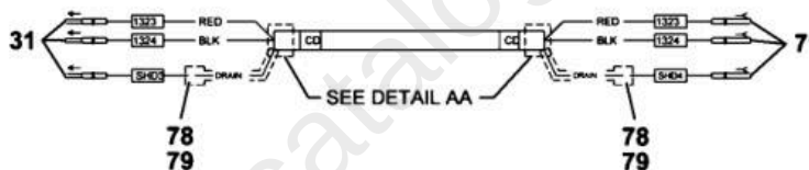
CABLE DETAIL CD CARRIER CONTROL MODULE-DIAGNOSTIC CABLE
