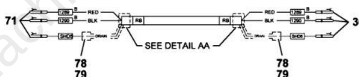
CABLE DETAIL RB J1939 ENGINE DATALINK CABLE
