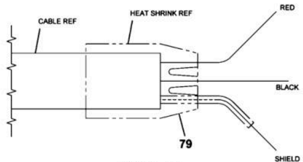
DETAIL AA
